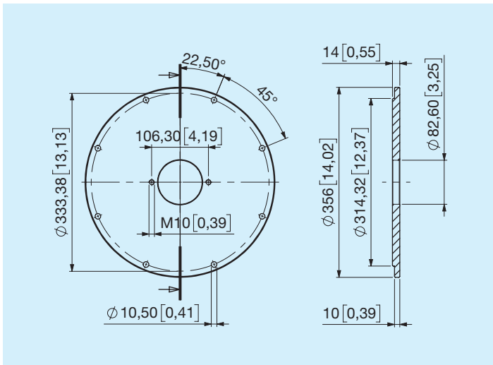
AAA SAE 5 A - 2 M10 holes
