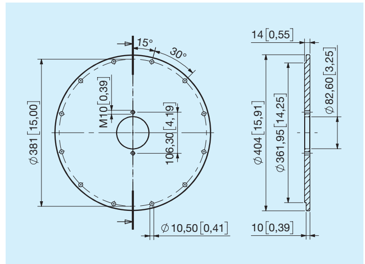
AAB SAE 4 A - 2 M10 holes
