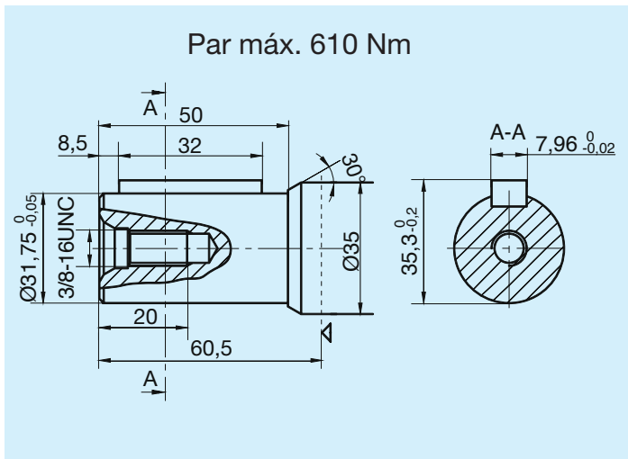
AP6 1 1/4" lengüeta BS46 5/16"x5/16"x1 1/4"
