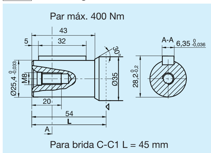
AP3 1" EU lengüeta BS46 1/4"x1/4"x1 1/4"
