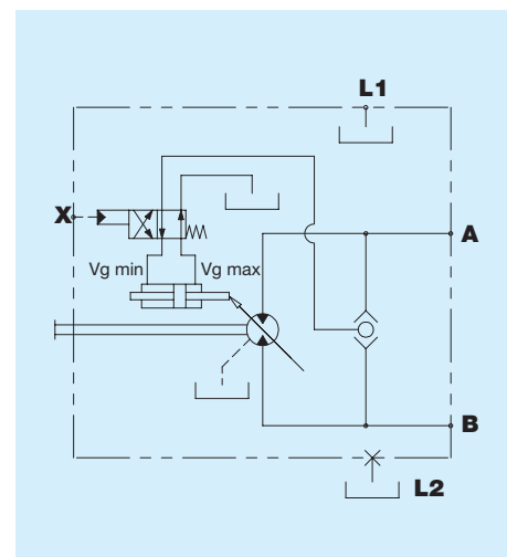
Hydraulic diagram
